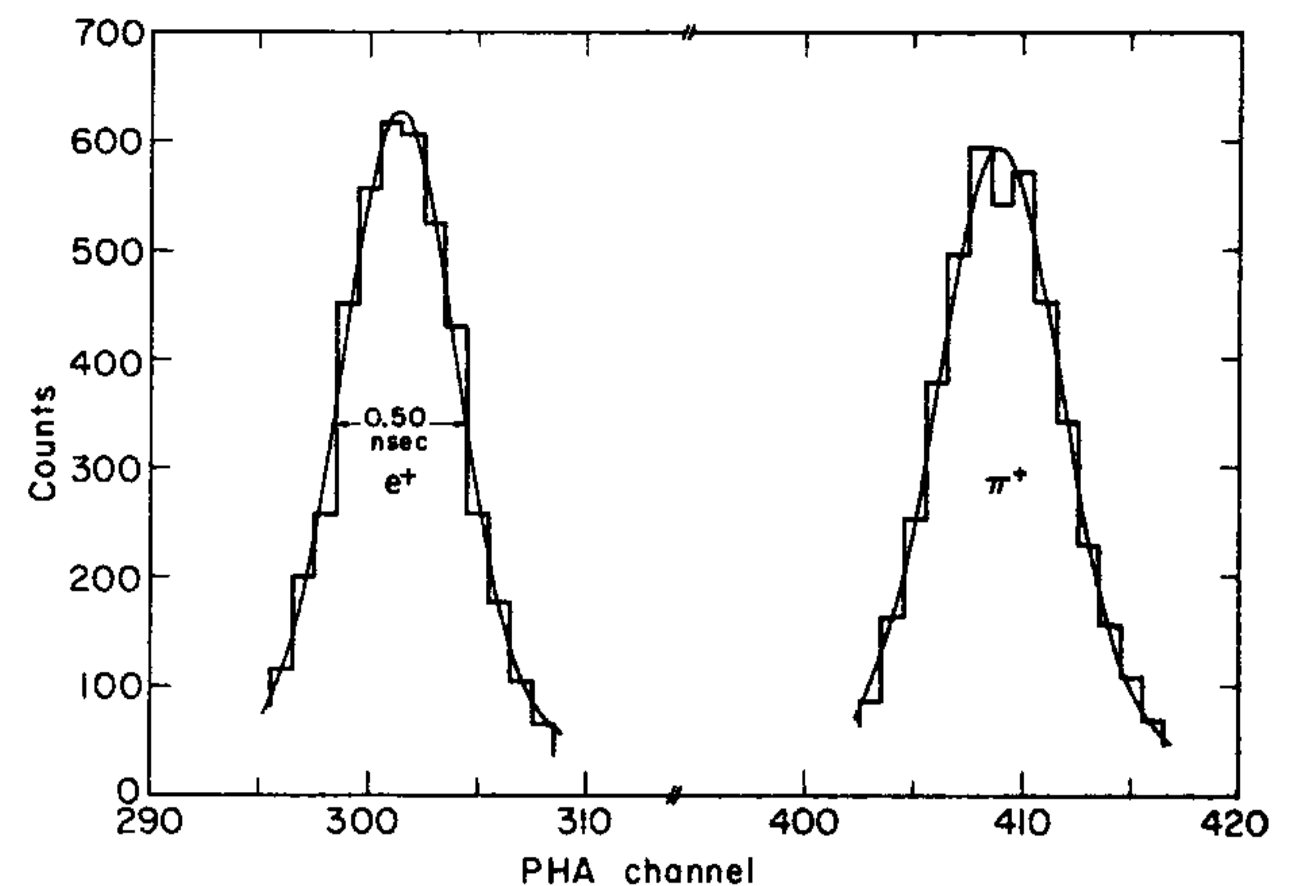
FIG. 2. Typical time-of-flight spectrum. Each fitted curve is a Gaussian plus constant background.
