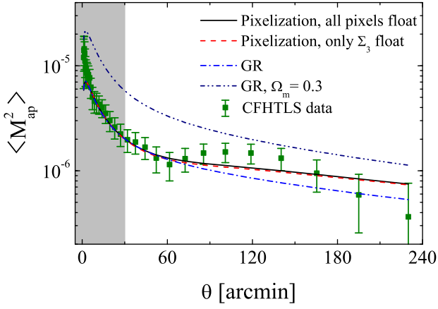
FIG. 8: Best-fit aperture mass power spectra \langle M_{\text{ap}}^2 \rangle for different MG parametrizations shown in different colors and line styles. Black solid: parametrization \mathcal{X}_{II} with all the pixels varying; Red dashed: parametrization \mathcal{X}_{II} with only \Sigma_3 varying; Blue dashed-dotted: GR; Navy dashed-dotted-dotted: GR with a fixed \Omega_m = 0.3 . The data points with error bars show the CFHTLS data; the shaded region is excluded from our analysis.
