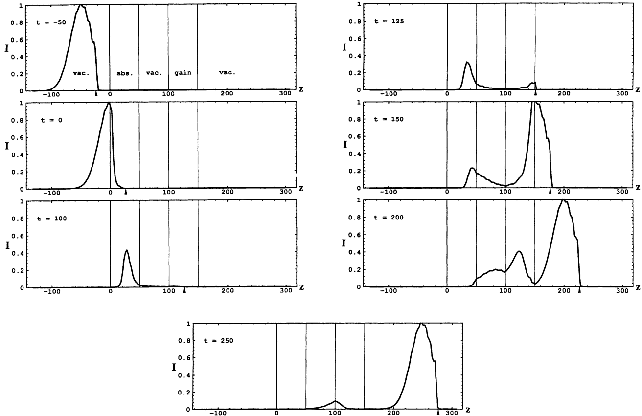
FIG. 4. Same configuration as for Fig. 3, but the Gaussian is step modulated; the step occurs at 1/e point of intensity. Graphs are based on numerical simulations. The location of the front ( z = ct ) is indicated by the pointer at each time. (Ripples near the step are due to numerical error.)
